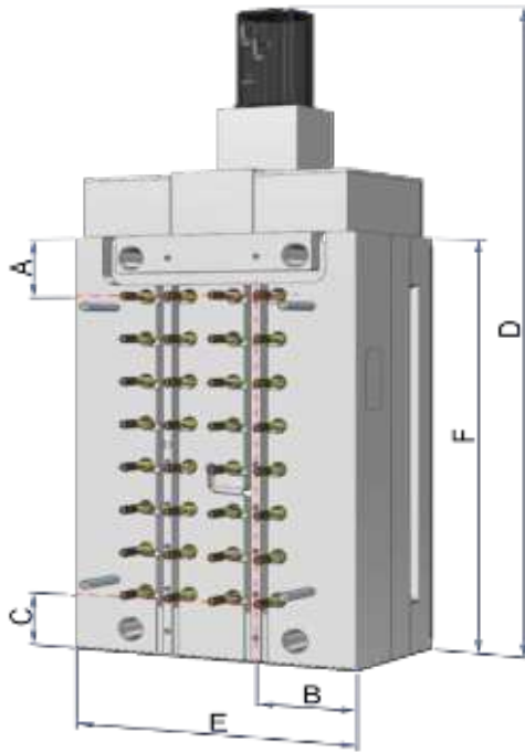
UltraSync E Plate and Space Requirements
