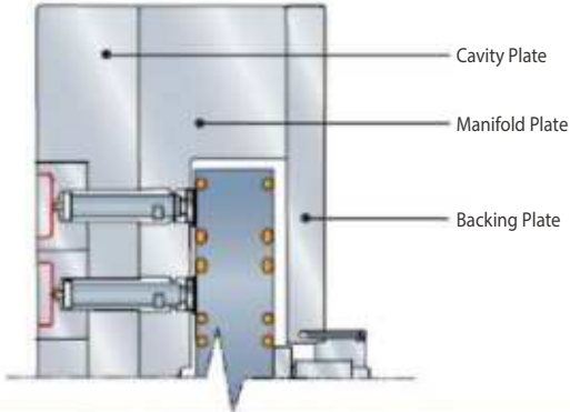
Integrated Manifold and Cavity Plate
