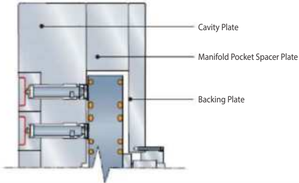
Manifold Pocket Spacer Plate
