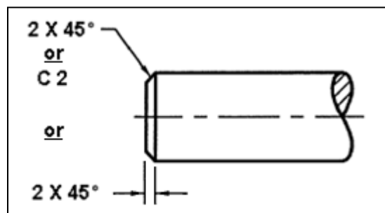
Figure 1-43 45° Chamfer [REPLACE]
