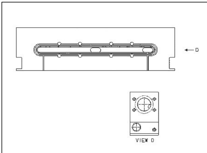
Fig. 1-7 - Removed Views [REPLACE]
