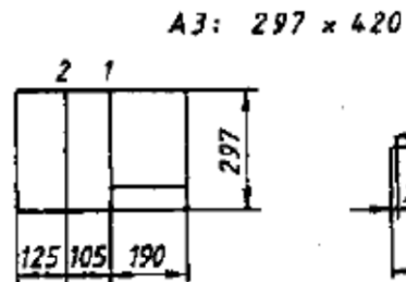
Figure 10 - Hand Folding Form A with Binding Margin
