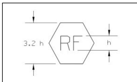
Fig. 3-31 - Size and Proportions of Restrained Feature Symbol [NEW]
