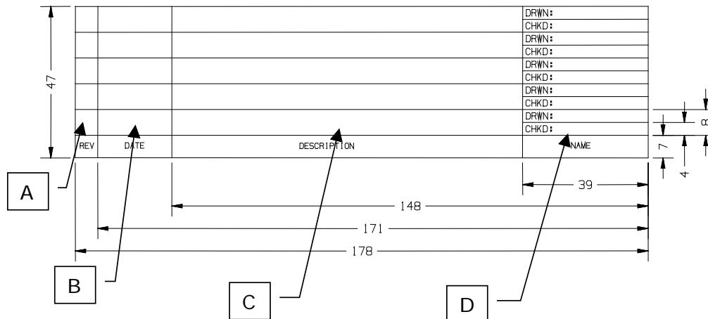
Figure 5 - Revision Block with Description
